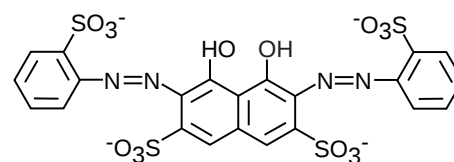
sulfonazo III (solution color : red purple)
