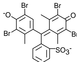
bromocresol green (bcg 2- ) (solution color : blue)
