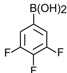
3,4,5-trifluorophenylboronic acid
