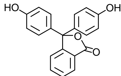
phenolphthalein (H 2 PP) (solution color : colorless)
