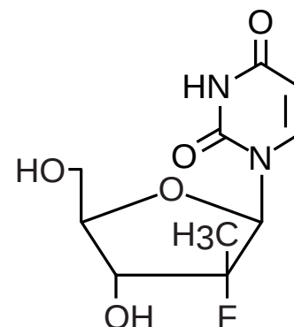
PSI-6206 ((2'R)-2'-deoxy-2'-fluoro-2'-methyluridine)
