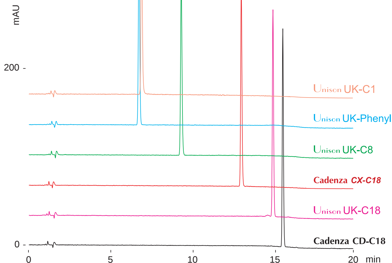
2,4,6-triphenyl-1,3,5-triazine
