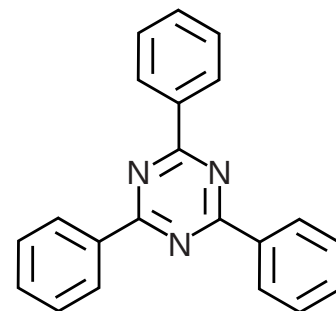
2,4,6-triphenyl-1,3,5-triazine
