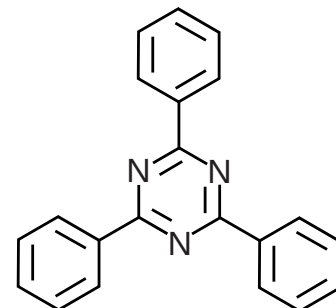
2,4,6-triphenyl-1,3,5-triazine
