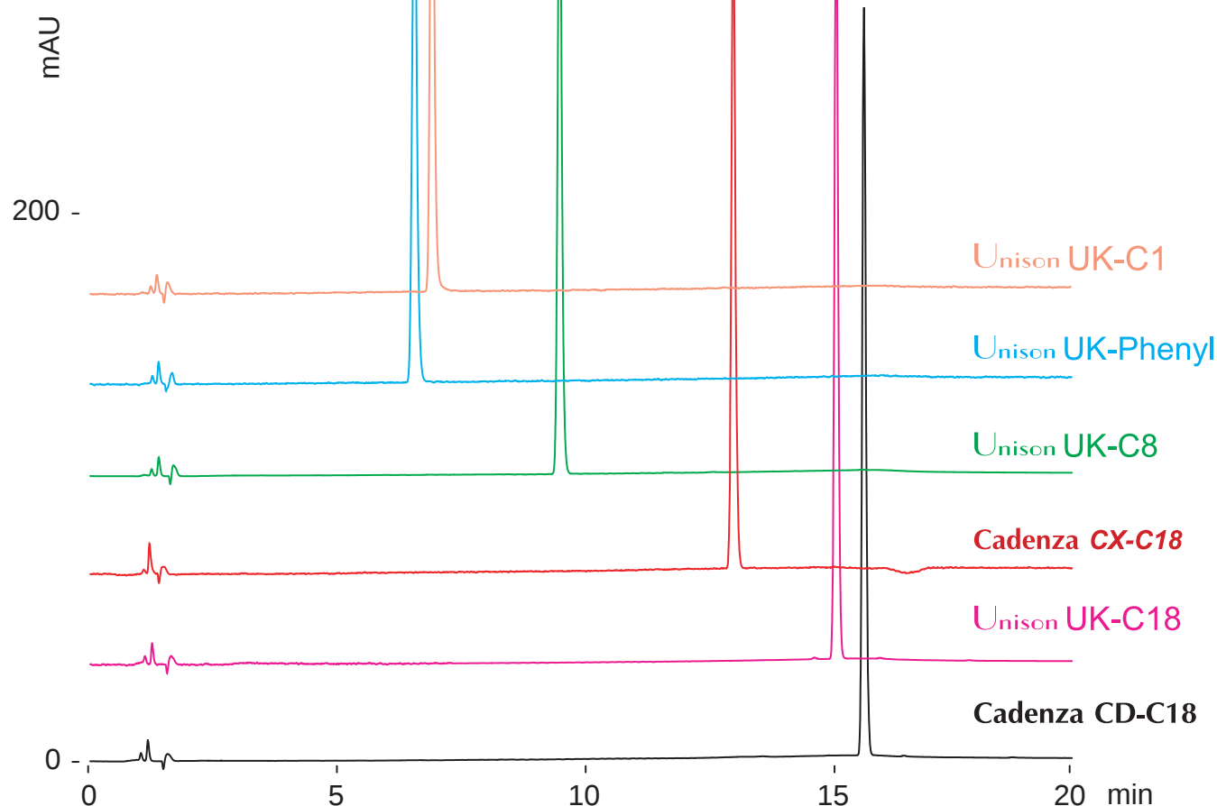
2,4,6-triphenyl-1,3,5-triazine
