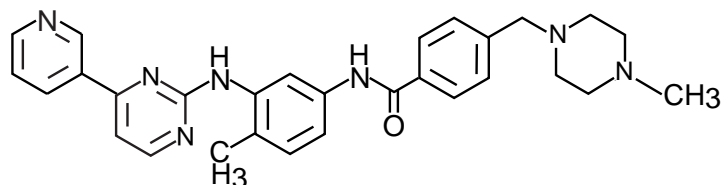
Imatinib
