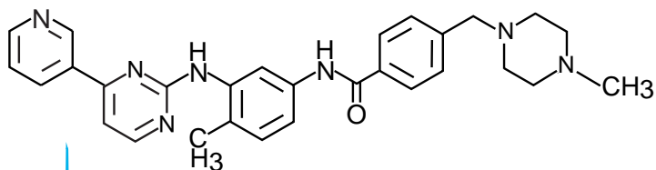
Imatinib
