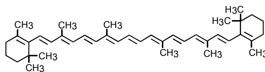
2 beta-carotene
