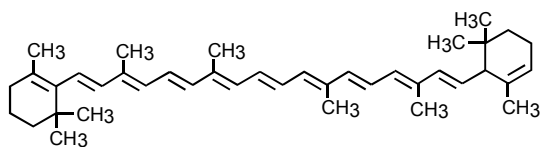
1 alpha-carotene
