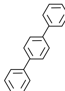
p -terphenyl
