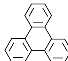
triphenylene
