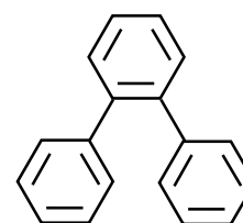
o -terphenyl
