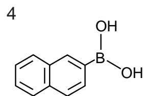
2-naphthaleneboronic acid
