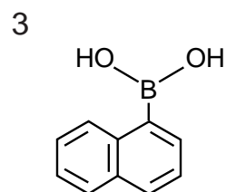
1-naphthaleneboronic acid
