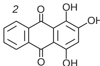
purpurin
