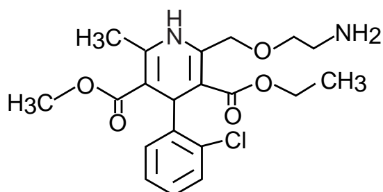
1. amlodipine
