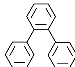
1 o -terphenyl
