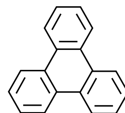
2 triphenylene
